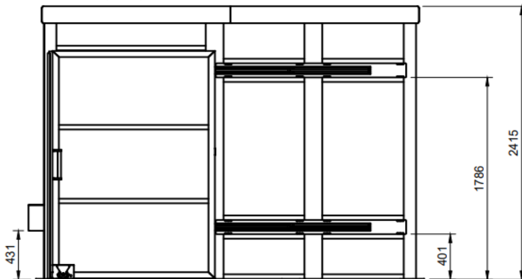
VIEW B (1 : 30)
